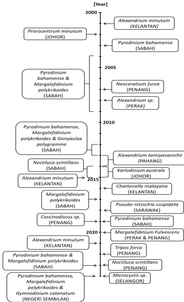
FIGURE 2. Timeline trend of reported HAB species in Malaysia. Species occurrences are indicated by the scientific name followed by the state in parentheses (for example Alexandrium minutum (Kelantan))
