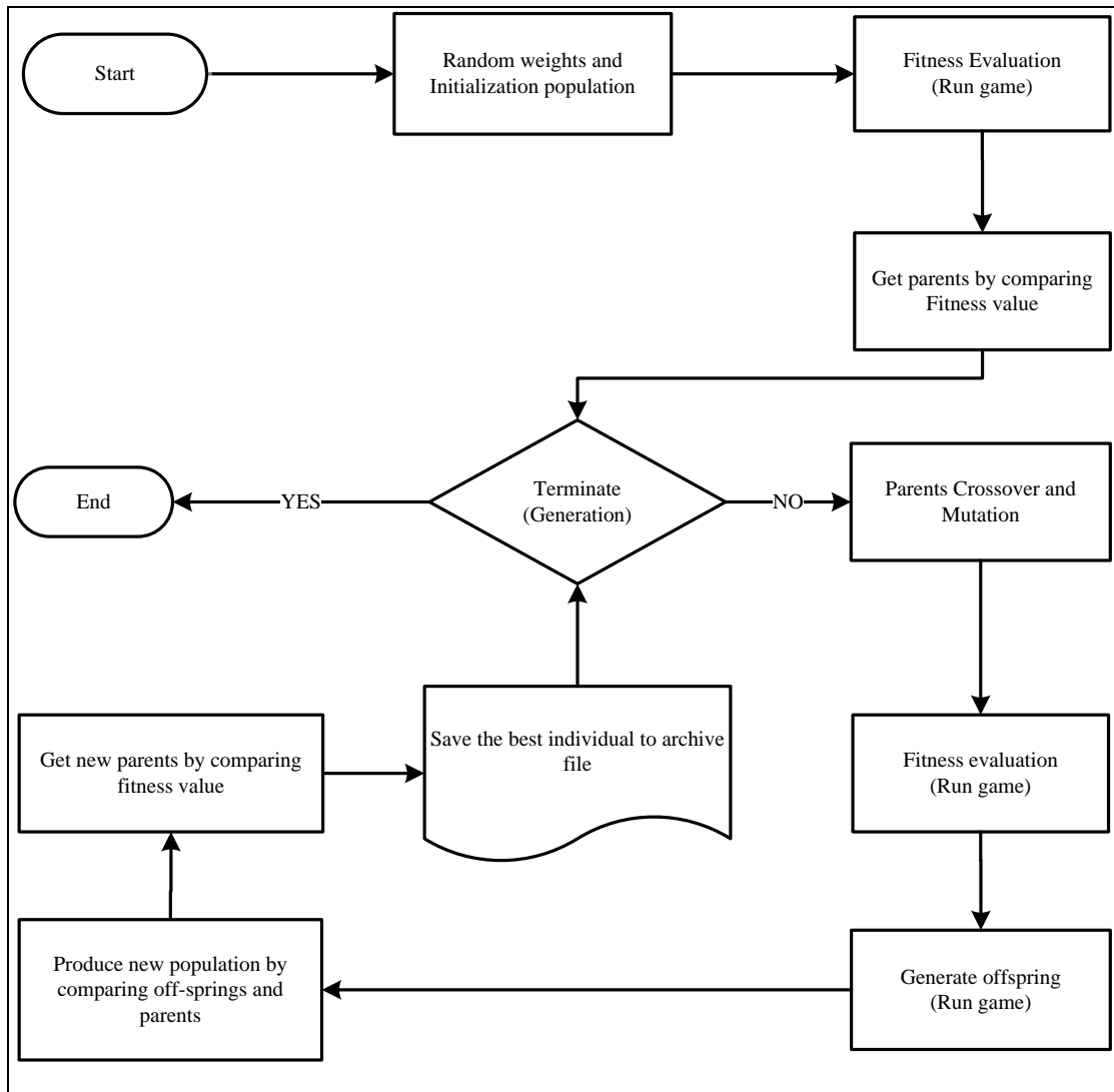
FIGURE 4. Flowchart of DE.
