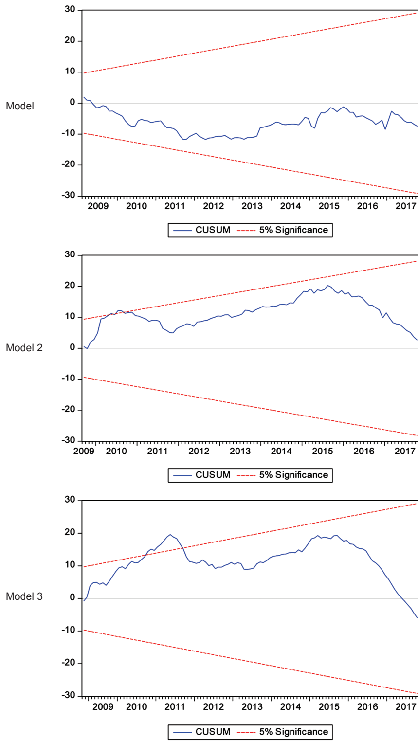
FIGURE 1. Recursive least square of CUSUM test
